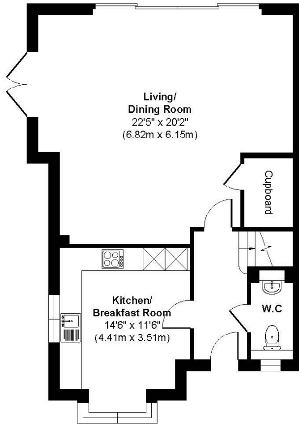
Ground Floor Approximate Floor Area 690 sq. ft (64.15 sq. m)
