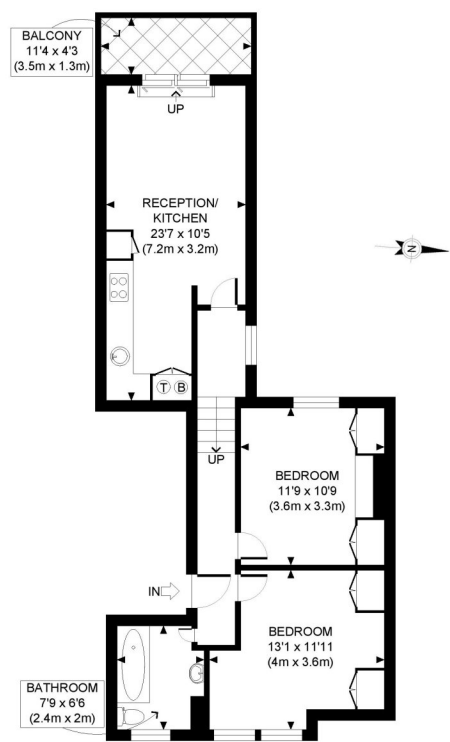
FIRST FLOOR GROSS INTERNAL FLOOR AREA 623 SQ FT
