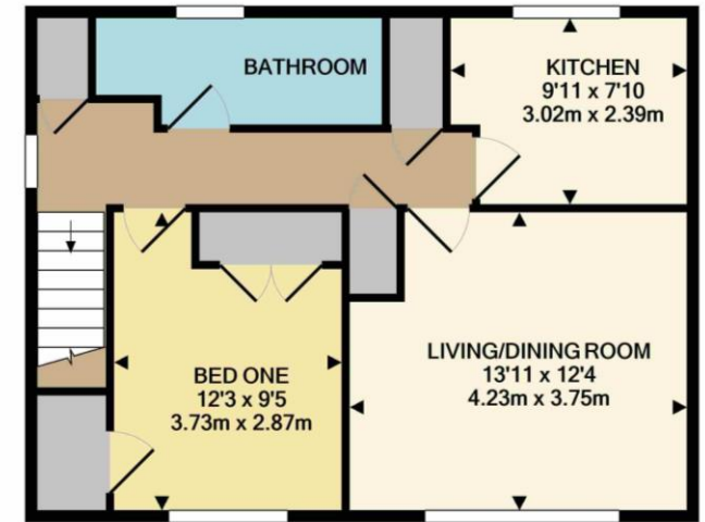
1ST FLOOR APPROX. FLOOR AREA 533 SQ.FT. (49.5 SQ.M.)
