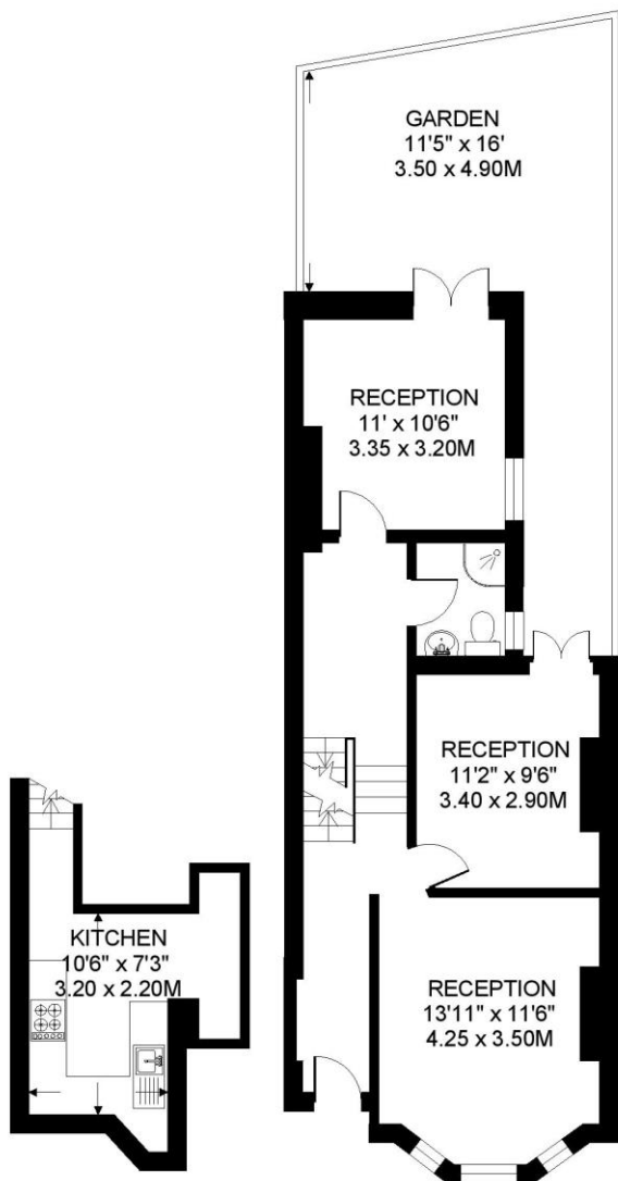
LOWER GROUND FLOOR 120 SQ.FT.
