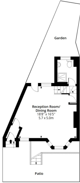
Upper Ground Floor Floor Area 393 Sq Ft - 36.51 Sq M
