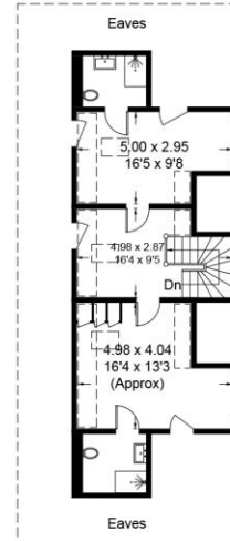
Second Floor
