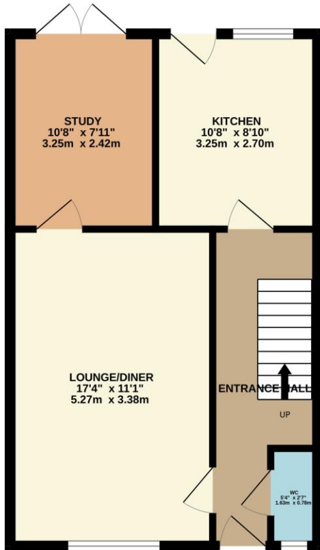
GROUND FLOOR 470 sq.ft. (43.7 sq.m.) approx.
