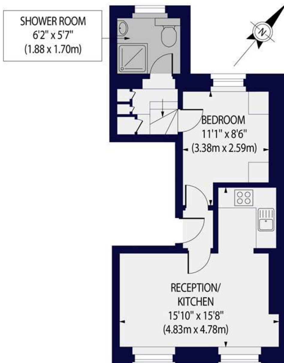
FIRST FLOOR
