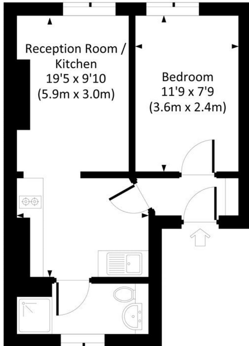
SECOND FLOOR
