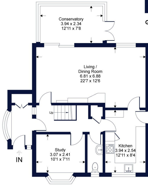
Ground Floor = 70.6 sqm / 760 sqft
