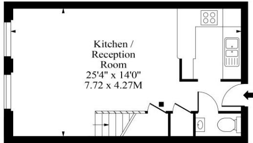
Fourth Floor
