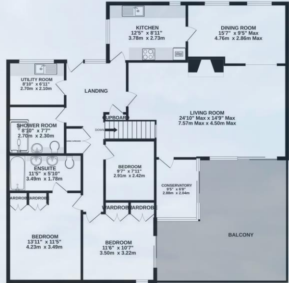
GROUND FLOOR 1387 sq.ft. (128.9 sq.m.) approx.
